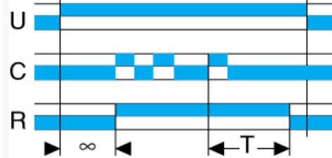
Function N - 1 relay output
